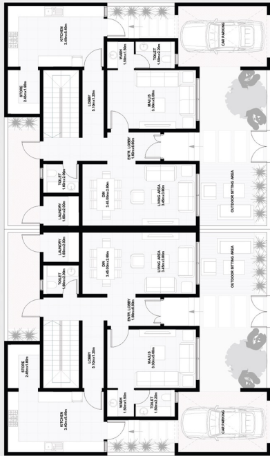
GROUND FLOOR PLAN 230.00sq.m
